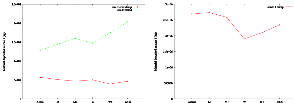
Figure 10: Amount of material deposited on the bottom at the end of the simulation in zone 1 around the fair channels for the different climate change scenarios (a) Left: simulations 1: hourly dumps & simulation 3: boundary conditions (b) Right: simulation 2: one dumping.
